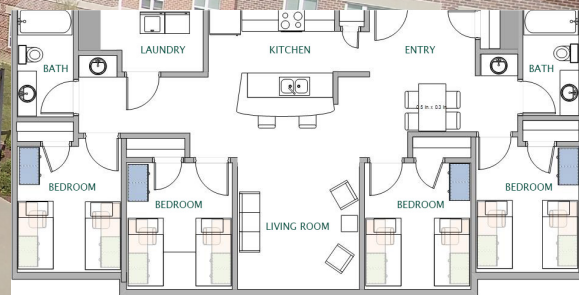
four bedroom suite floorplan
